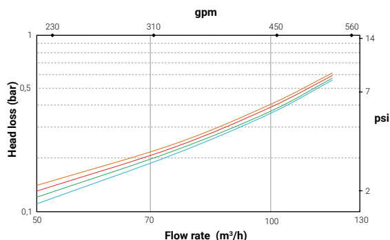
HEAD LOSS PER FILTRATION DEGREE*
